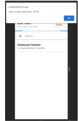
Gambar 24 Generate Token
