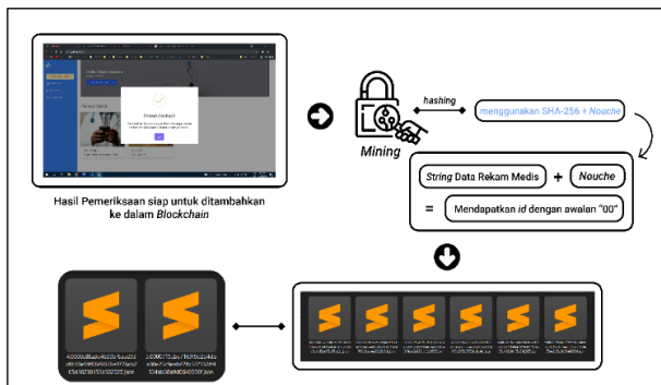
Gambar 13 Alur Mining
