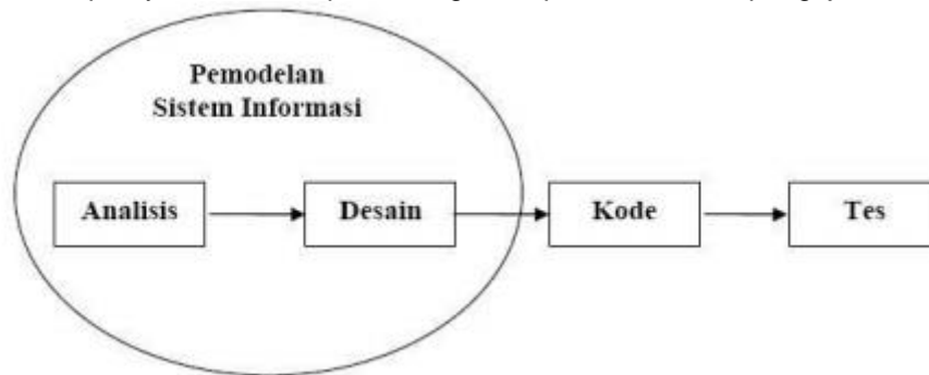
Gambar 1. Model waterfall
